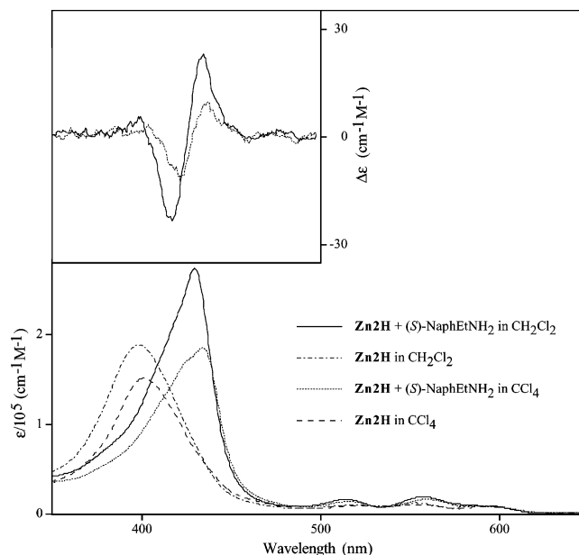
Figure 5. UV-vis and CD (inset) spectra of Zn2H with and without ( S )-NaphEtNH 2 in CH 2 Cl 2 and CCl 4 at 293 K.
