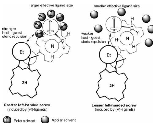
SCHEME 5: Schematic Representation of the Solvent Effect on Supramolecular Chirality Induction in Zn2H•L*
