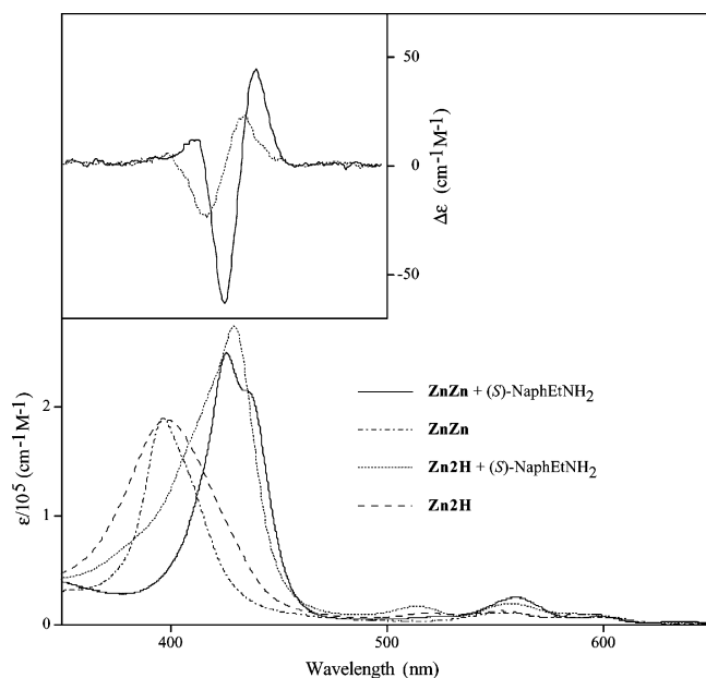
Figure 3. UV-vis and CD (inset) spectra of \text{ZnZn} and \text{Zn2H} with and without (S)\text{-NaphEtNH}_2 in \text{CH}_2\text{Cl}_2 at 293 K.
